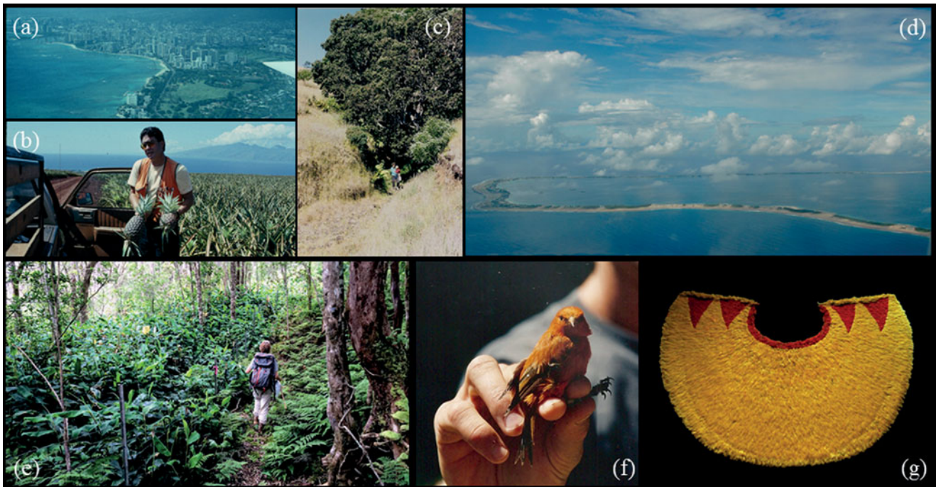
Figure 2 Examples of major threats to island ecosystems, with illustrations from the Hawaiian Islands and Micronesia. (a) Urban development. Aerial photo of Honolulu, showing the entirely modified urban environment of Waikiki. The initial wetlands were first modified in the mid-15th century to cultivate wetland taro and for fishponds, then they were drained in the 1920s with construction of the Ala Wai Canal to mitigate mosquito-borne human disease with further urbanization. Photo credit: George K. Roderick. (b) Crops. Pineapples, with sugar, were major plantation crops in Hawai'i starting in the mid-1800s (Perroy et al. 2016). Acreage in pineapple and sugar halved between 1980 and 2015 and Maui Land and Pineapple Company (shown here) closed in 2009. Currently, many plantations lie idle and weed ridden, with an uncertain future. Photo credit: George K. Roderick. (c) Pasture. Cattle were introduced into the Hawaiian Islands in the 1790s, and ranching started in the early-to-mid-1800s, and patches of native forest became increasingly restricted to inaccessible gulches, as shown in this photo of Hakalau Forest National Wildlife Refuge. Recent efforts are restoring areas of degraded pasture and forest, such as those at Auwahi on Maui (Cabin 2013). Photo credit: George K. Roderick. (d) Climate change. The many atolls that make up Micronesia now suffer frequent inundation as a result of sea level rise, as illustrated in this photo of Majuro in the Marshall Islands, which has become a vocal participant in global climate change discussions (Labriola 2016). Many low-lying island nations of the Pacific are buying tracts of land on higher islands (Green 2016). Photo credit: George K. Roderick. (e) Invasions. One of the most insidious invaders of native ecosystems in the Hawaiian Islands is kahili ginger, Hedychium gardnerianum (The Nature Conservancy of Hawaii 2011), as shown: the left side shows a monotypic stand of ginger, the right a relatively pristine forest. The fence in front of the ginger, marking the boundary of the Waikamoi Preserve, in no way inhibits the spread, which is controlled to the extent possible by the diligence of The Nature Conservancy of Hawaii employees. Photo credit: George K. Roderick. (f) Disease. Studies, such as that which is shown here at Hakalau Forest National Wildlife Refuge, show that native honeycreepers such as the 'apapane are vulnerable to pox and malaria (LaPointe 2008) and might be affected by upslope expansion of avian diseases (Camp et al. 2010). Photo credit: George K. Roderick. (g) Direct exploitation. In the Hawaiian Islands, the strongest evidence of direct exploitation is the use of native bird feathers in capes. Perhaps most dramatic was the 'O'o, which was common in the 1800s, but was extinct by the mid-1900s, and was exploited for a small tuft of yellow shoulder feathers (Lovette 2008). Photo credit: Honolulu Museum of Art.
