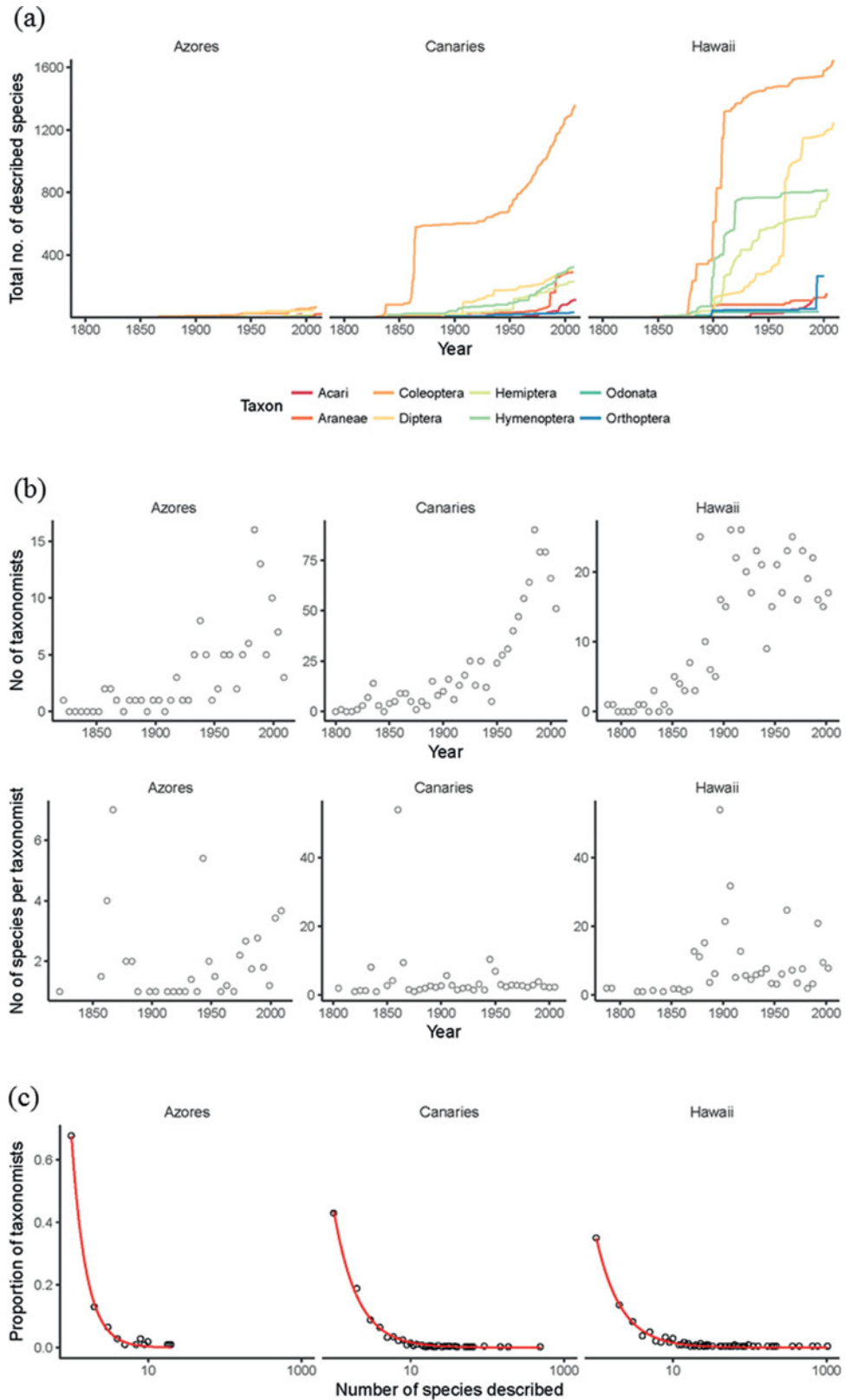
Figure 3 Temporal trends in taxonomic description and taxonomic effort. (a) Cumulative number of described species over time for various arthropod orders for the Azorean, Canarian and Hawaiian archipelagos. Data were obtained from recent arthropod checklists (Nishida 2002; Borges et al. 2005). (b) Trends over time (5-year bins) in the number of taxonomists and the number of species described per taxonomist. (c) Distribution of species descriptions among taxonomists. Most taxonomists describe few species, but there are fewer singletons (taxonomists that describe only one species) on Hawai'i. The lines represent non-parametric smoothed best-fit lines (LOESS regression).
