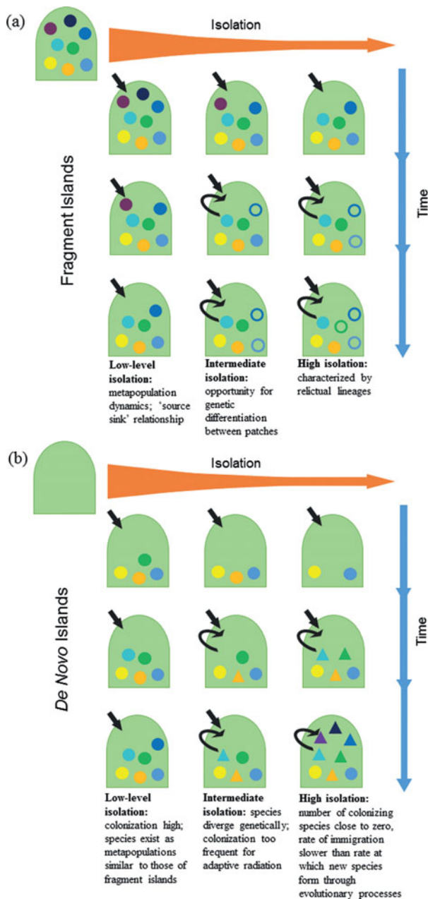
Figure 1 Evolutionary assembly of de novo and fragment islands at varying levels of time and isolation. Differently shaded shapes represent species as they accumulate through colonization and through the formation of new species by both processes of anagenesis and cladogenesis. Black arrows indicate whether species are primarily accumulated by colonization (incoming arrow) or genetic divergence (arching arrow). (a) Fragment islands begin with biota similar to source. The number of species will decrease over ecological time as a result of relaxation and simply because of reduced area. Over evolutionary time, species diverge from original stock through anagenesis (unfilled circles), with the formation of paleo-endemics. (b) De novo islands are formed without life, thus the ecological space is open and available when they first appear. Over time, species increase through both colonization and the formation of new species by cladogenesis (triangles). At high isolation, multiple neo-endemics may form through adaptive radiation.
